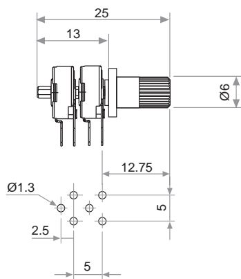
Fig. 18 - Ref: 6064 2-gang plastic knob/shaft
