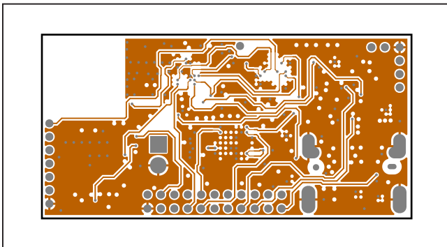
MAXSENSORBLE_EVKIT_B PCB Layout Diagrams—Internal 10
