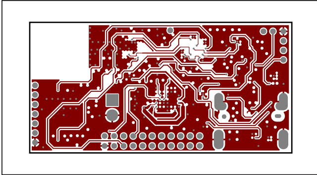
MAXSENSORBLE_EVKIT_B PCB Layout Diagrams—Internal 6
