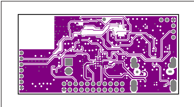
MAXSENSORBLE_EVKIT_B PCB Layout Diagrams—Internal 8
