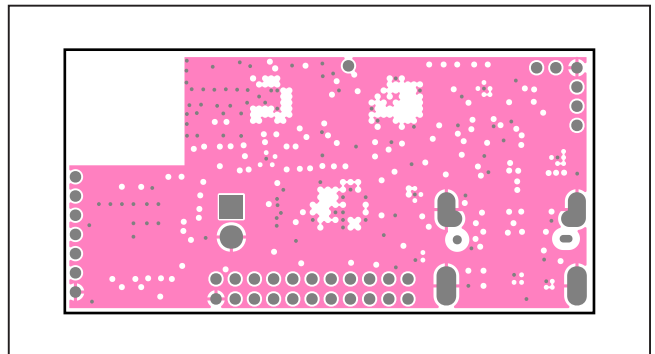
MAXSENSORBLE_EVKIT_B PCB Layout Diagrams—Internal 11
