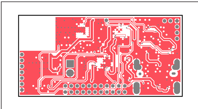
MAXSENSORBLE_EVKIT_B PCB Layout Diagrams—Internal 4
