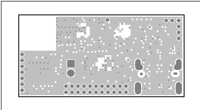
MAXSENSORBLE_EVKIT_B PCB Layout Diagrams—Internal 2
