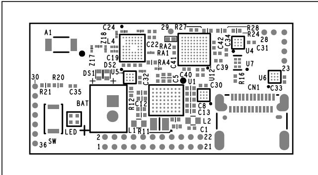
MAXSENSORBLE_EVKIT_B Component Placement Guide— Top Silkscreen
