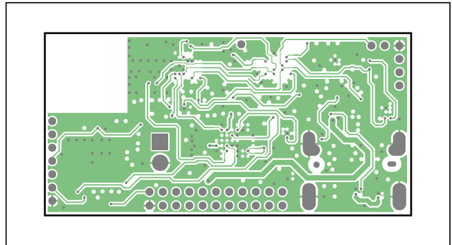
MAXSENSORBLE_EVKIT_B PCB Layout Diagrams—Internal 3
