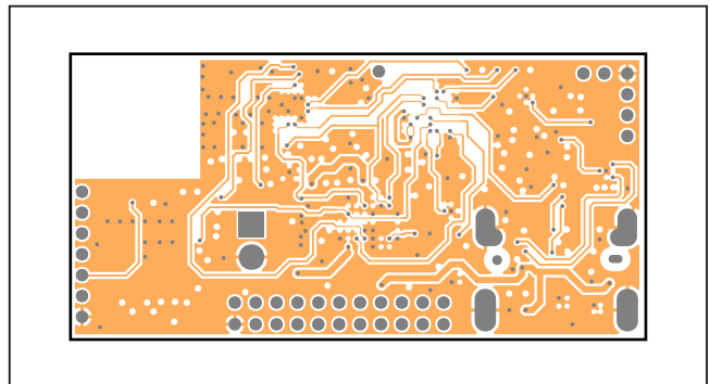
MAXSENSORBLE_EVKIT_B PCB Layout Diagrams—Internal 5
