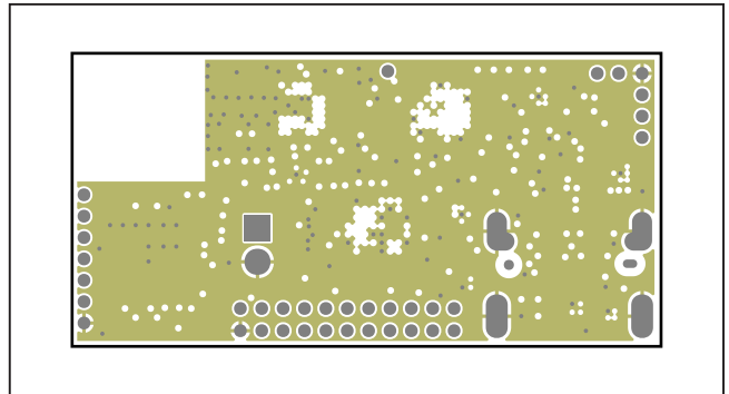
MAXSENSORBLE_EVKIT_B PCB Layout Diagrams—Internal 9
