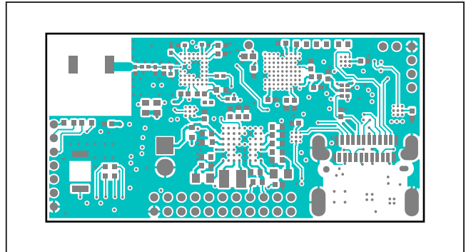
MAXSENSORBLE_EVKIT_B PCB Layout Diagrams—Top View
