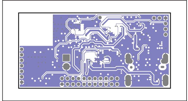
MAXSENSORBLE_EVKIT_B PCB Layout Diagrams—Internal 7
