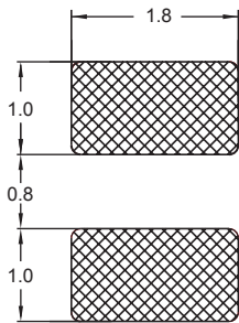
recommended layout for solder pads
