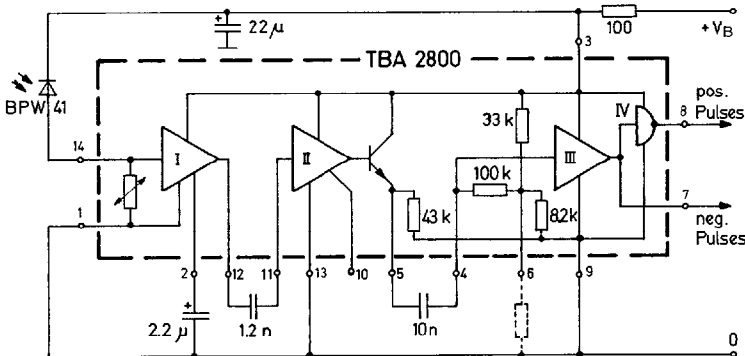
Fig. 1: TBA 2800 block diagram and application circuit
