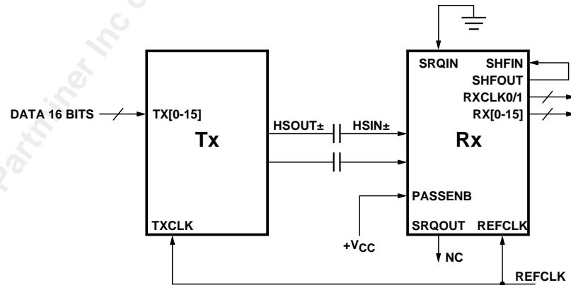
Figure 4.2. Single channel configuration with PASS enabled (PASSENB=1). Recovered data words and RXCLK0/1 are synchronous with REFCLK.
