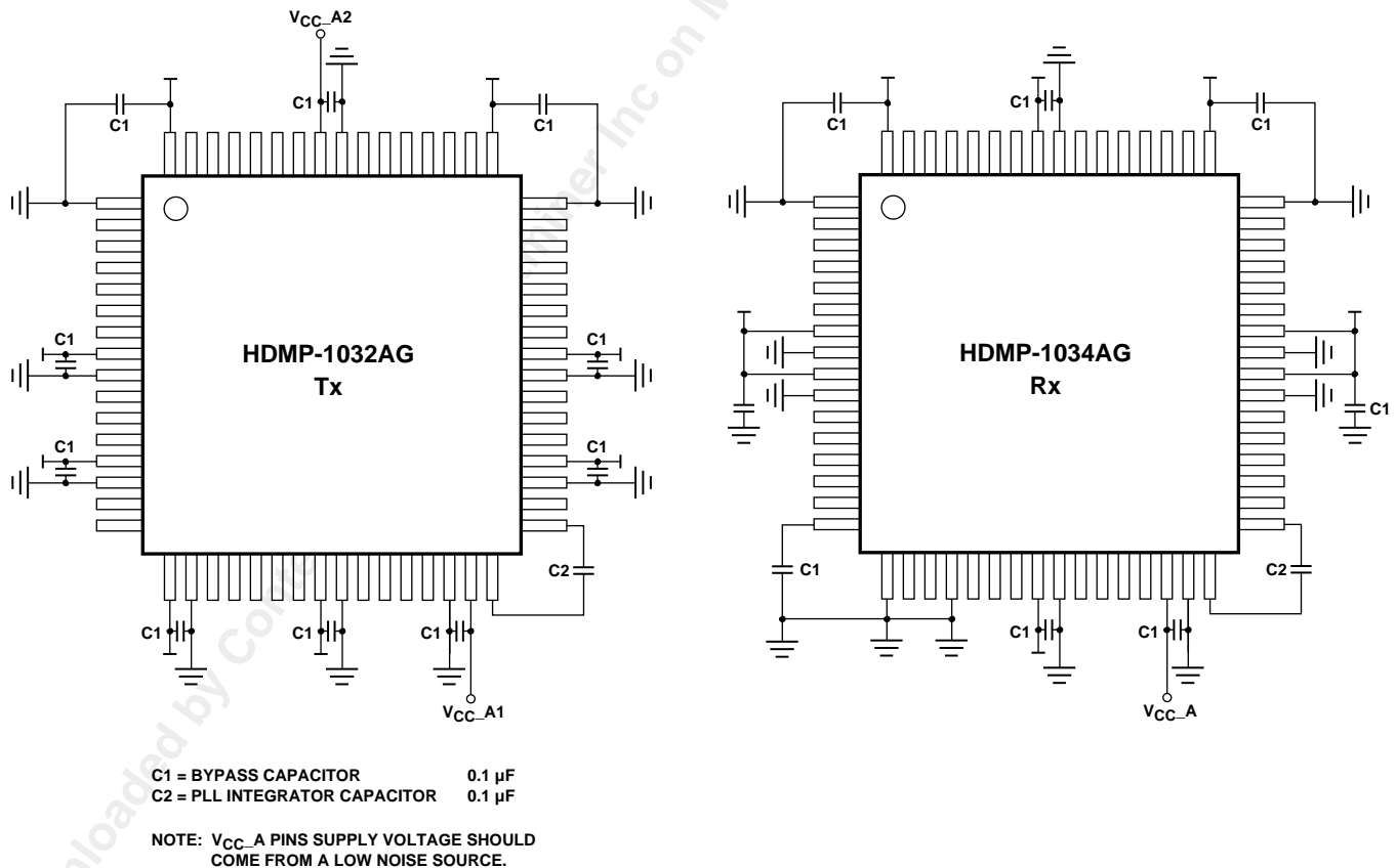
Figure 12. HDMP-1032AG (Tx) and HDMP-1034AG (Rx) power supply pins.
