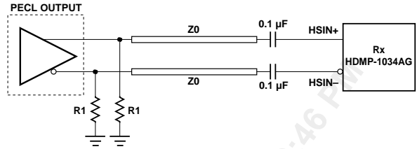
C) GENERIC PECL OUTPUT TO G-LINK Rx INPUT
