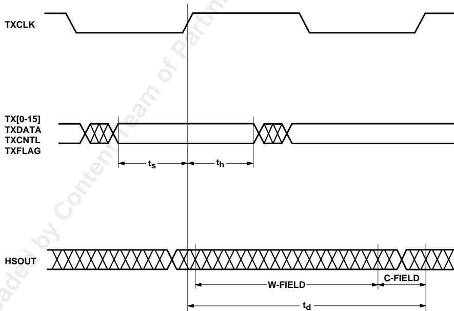
Figure 5. HDMP-1032AG (Tx) timing diagram.
