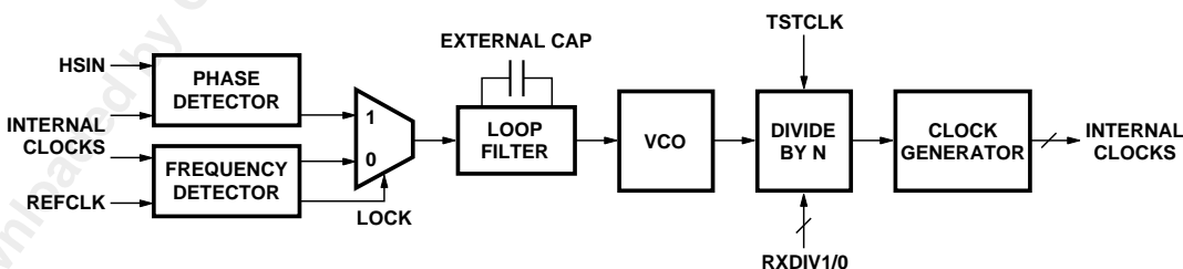
Figure 11. HDMP-1034AG (Rx) phase-lock loop.
