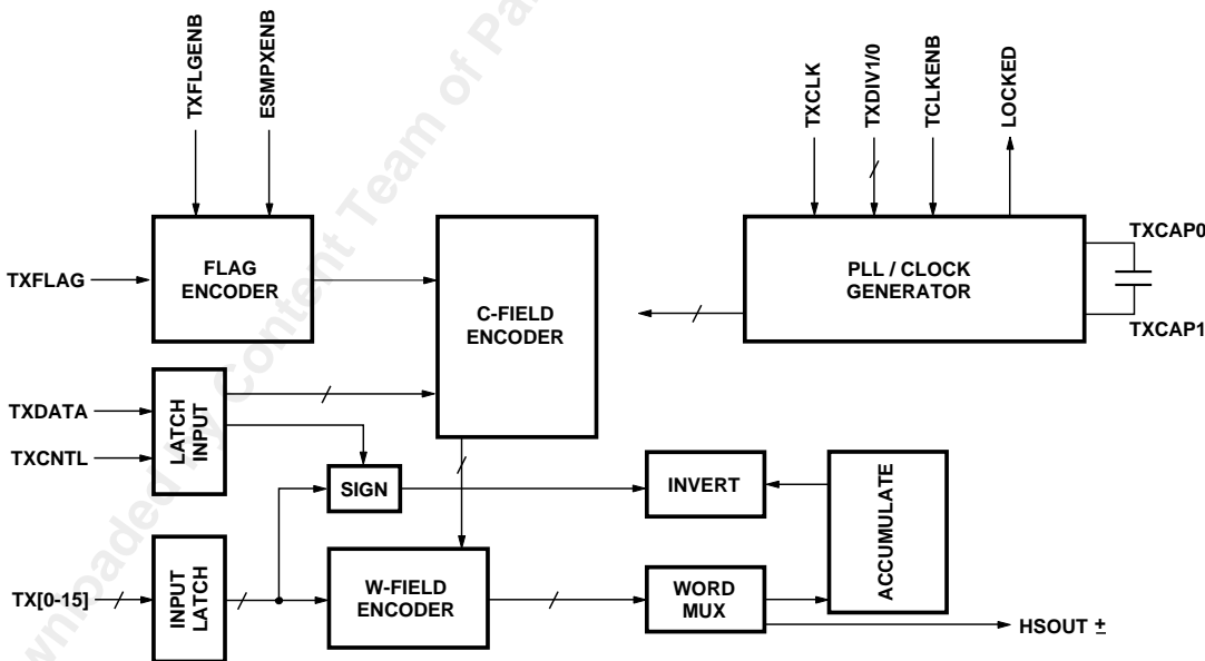
Figure 3. HDMP-1032AG transmitter block diagram.
