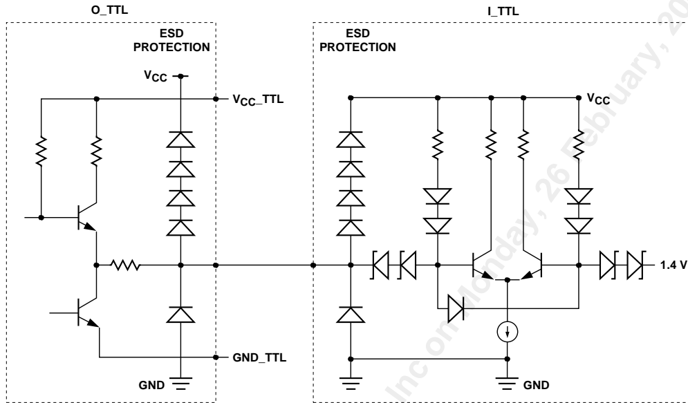
Figure 13. O-TTL and I-TTL simplified circuit schematic.
