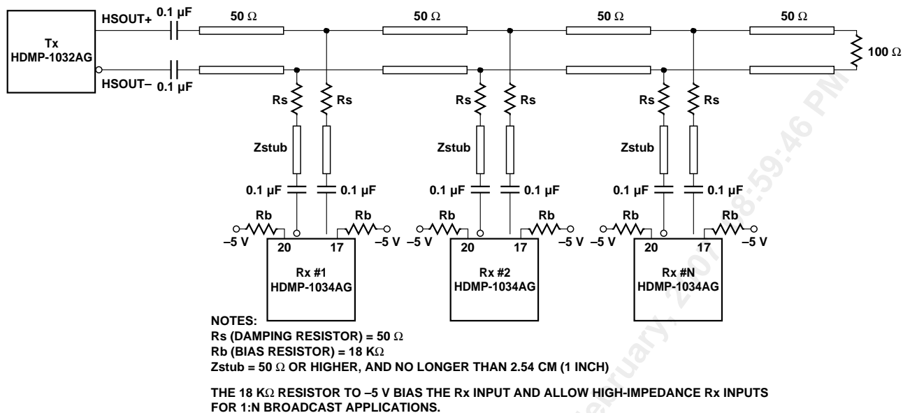
Figure 16. Data bus line transmission.
