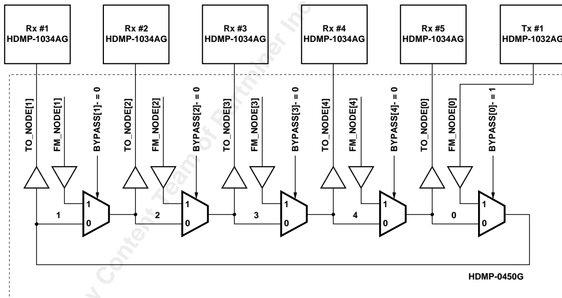
Figure 17. Broadcast transmission using an HDMP-0450G port-bypass circuit.
