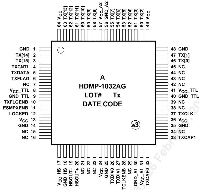
Figure 7. HDMP-1032AG (Tx) package layout, top view.
