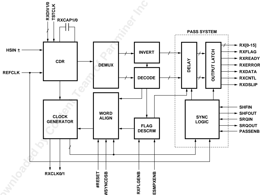
Figure 4. HDMP-1034AG receiver block diagram.
