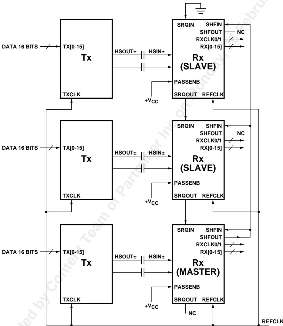
Figure 4.3. Multiple channel configuration with PASS Enabled (PASSEN=1).
