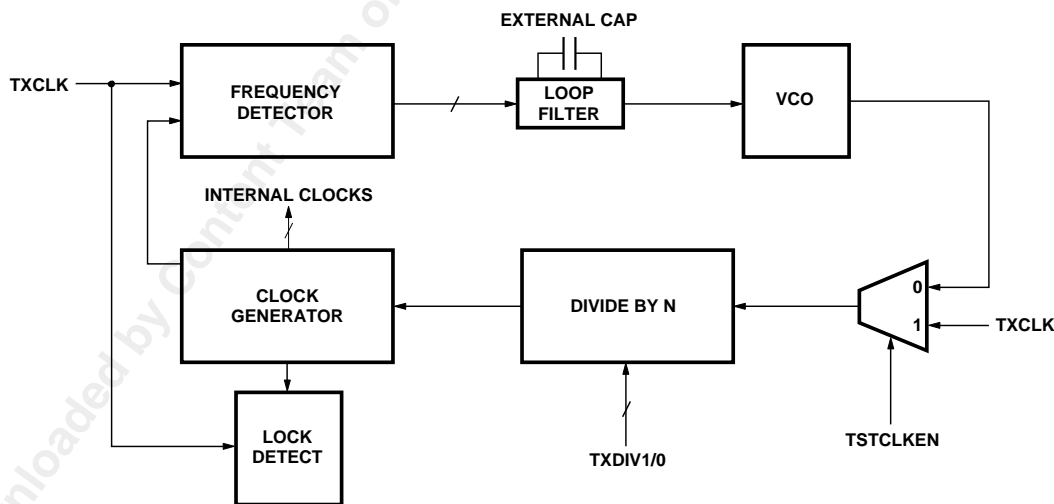
Figure 10. HDMP-1032AG (Tx) phase-lock loop.
