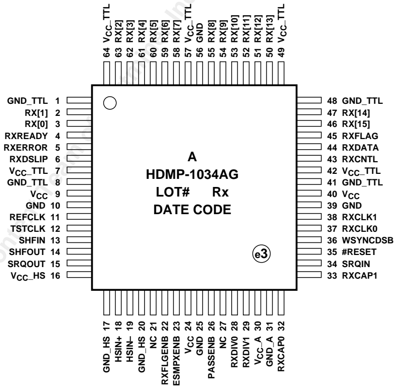
Figure 8. HDMP-1034AG (Rx) package layout, top view.
