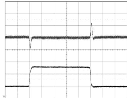
Output voltage response to load current step-change (7.5-22.5-7.5 A) at: T_{ref} = +25^\circ\text{C} , V_i = 53\text{ V} . Top trace: output voltage (200 mV/div.). Bottom trace: load current (10 A/div.). Time scale: (0.1 ms/div.).
