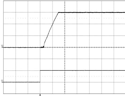
Start-up enabled by connecting V_i at: T_{ref} = +25^\circ\text{C} , V_i = 53\text{ V} , I_o = 30\text{ A} resistive load. Top trace: output voltage (0.5 V/div.). Bottom trace: input voltage (20 V/div.). Time scale: (5 ms/div.).
