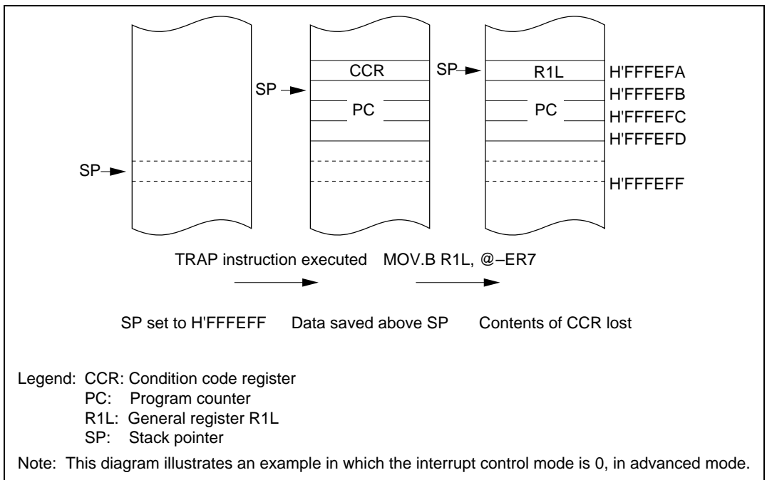
Figure 4.6 Operation when SP Value is Odd
