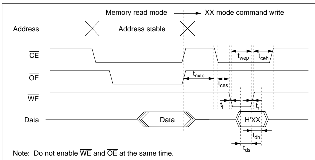
Figure 17.30 Timing Waveforms when Entering Another Mode from Memory Read Mode
