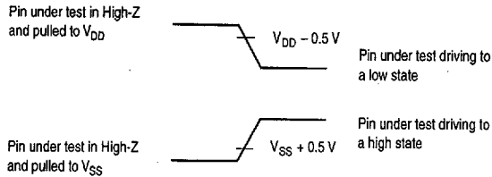
Figure 6-5. Test Point Levels for Three-State-to-Driven Time Measurements
