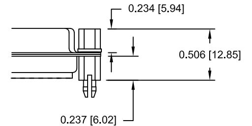
91X ..... 0.237" BOARD SIDE 0.197 MATING SIDE
