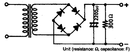
Specified Transformer Power Supply (Equivalent to RP-22)
