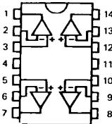
DIP14 CERDIP14 SO14
