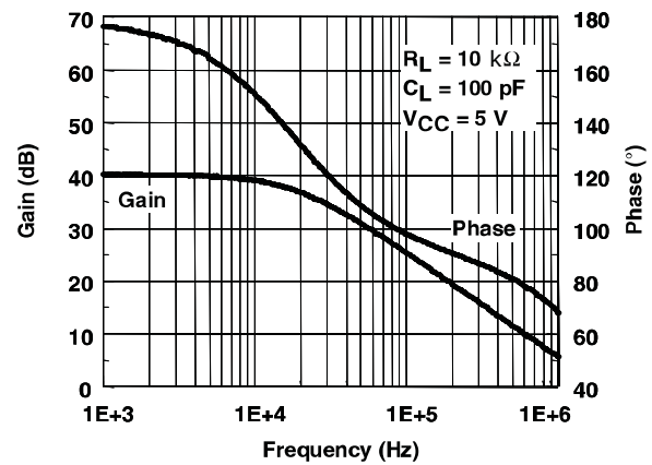
Figure 14: Gain and phase vs. frequency at V_{CC} = 5 V
