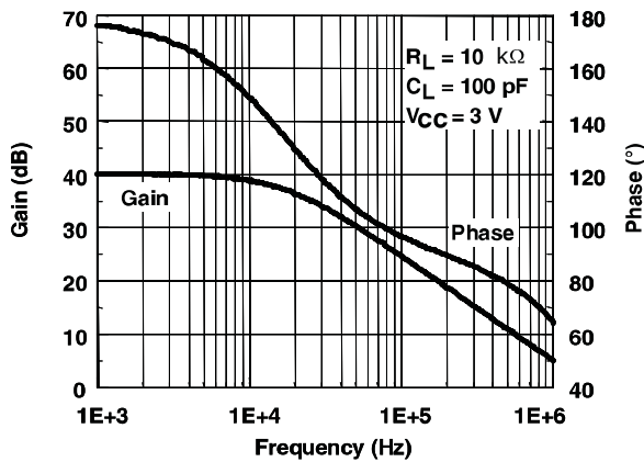
Figure 15: Gain and phase vs. frequency at V_{CC} = 3 V
