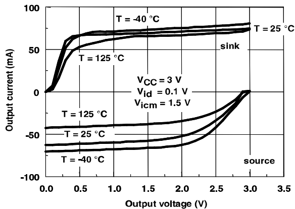
Figure 13: Output current vs. output voltage at V_{CC} = 3 V
