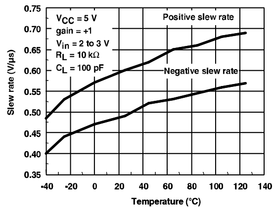
Figure 16: Slew rate vs. temperature at V_{CC} = 5 V
