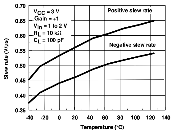
Figure 17: Slew rate vs. temperature at V_{CC} = 3 V
