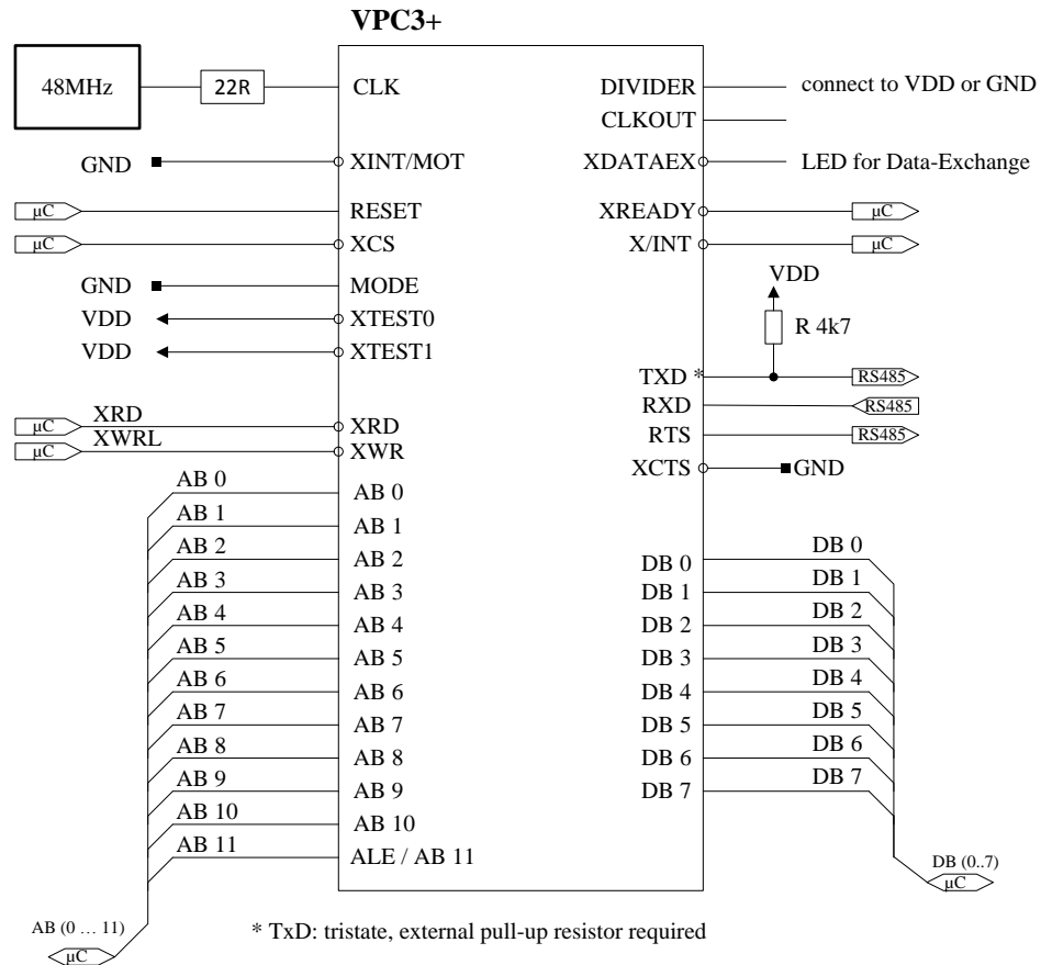
Figure 8-27: 80C165 Application
