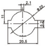
KCD1-103-8 ON-OFF-ON
