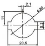
KCD1-101EN-8 ON-OFF
