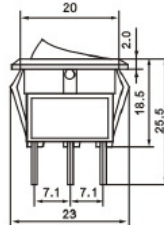
KCD1-103-8 ON-OFF-ON
