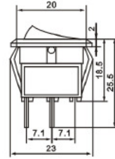
KCD1-103-8 ON-OFF-ON
