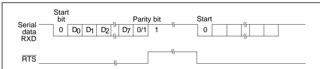
Figure 19.11 Example of Operation Using Modem Control ( \overline{\text{RTS}} )
