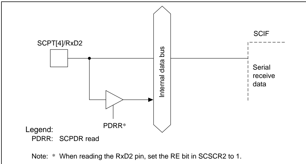
Figure 19.3 SCPT[4]/RxD2 Pin
