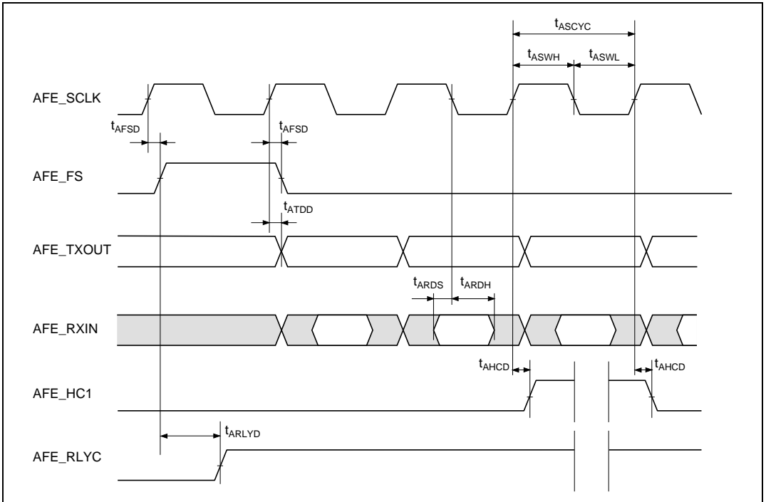
Figure 32.59 AFEIF Module AC Timing
