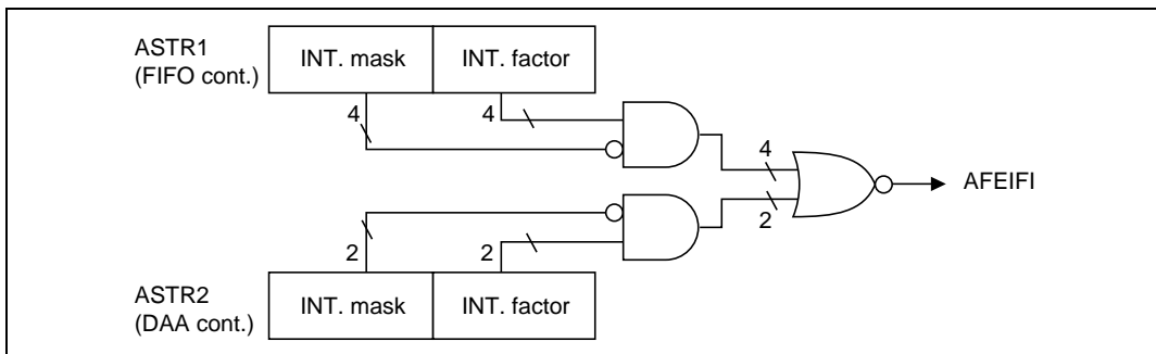
Figure 21.4 Interrupt Generator
