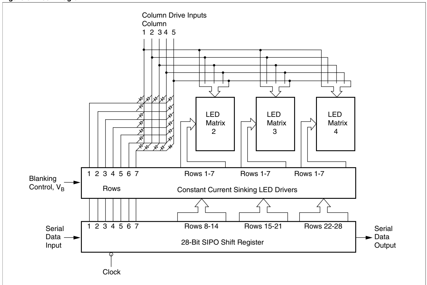
Figure 8. Block Diagram
