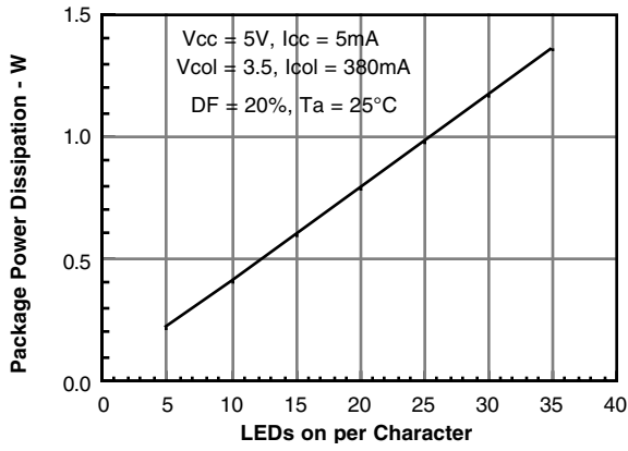
Figure 17. Max. Package Power Dissipation, ISD235X
