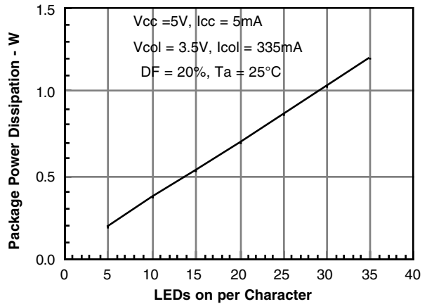
Figure 15. Package Power Dissipation, ISD201X
