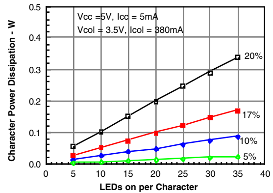
Figure 22. Character Power Dissipation, ISD231X
