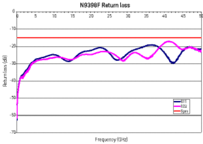
Figure 10. N9398F typical return loss versus frequency
