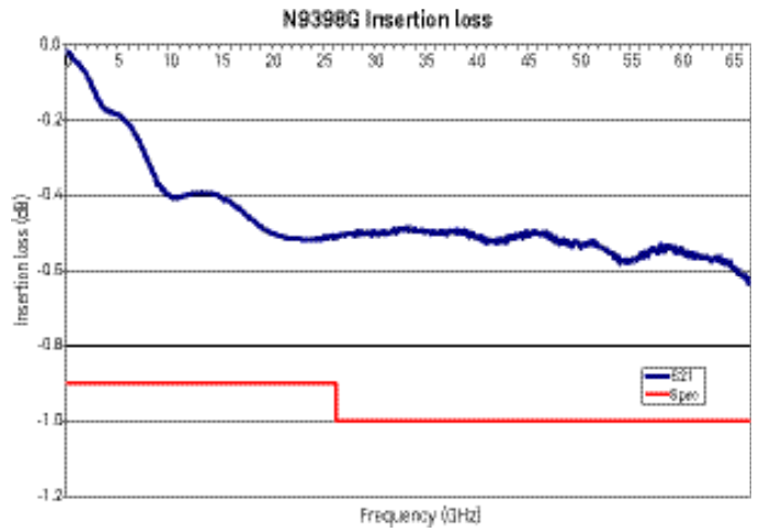
Figure 15. N9398G typical insertion loss versus frequency
