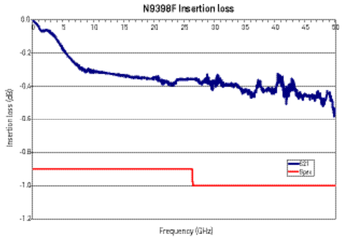
Figure 11. N9398F typical insertion loss versus frequency
