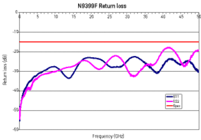
Figure 12. N9399F typical return loss versus frequency
