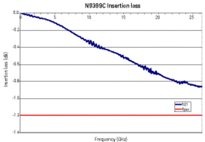
Figure 9. N9399C typical insertion loss versus frequency
