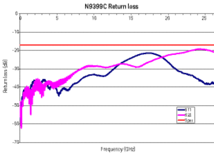
Figure 8. N9399C typical return loss versus frequency
