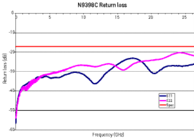
Figure 6. N9398C typical return loss versus frequency
