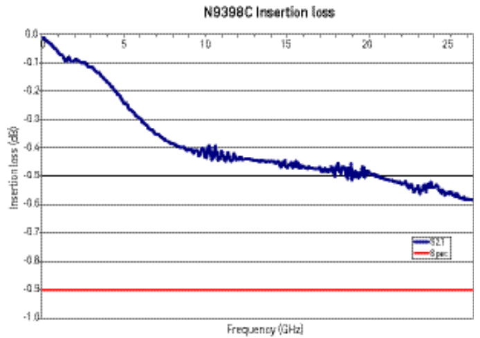
Figure 7. N9398C typical insertion loss versus frequency
