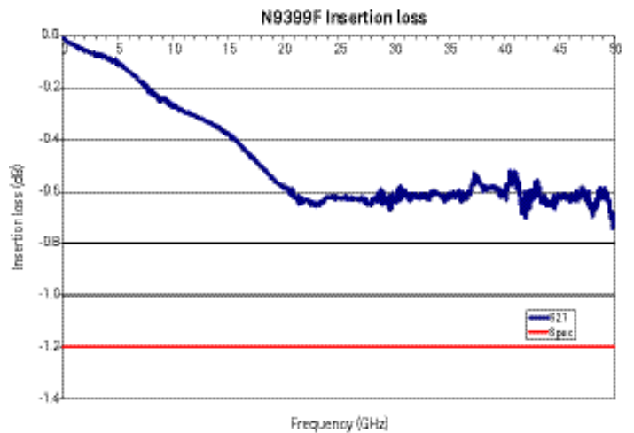
Figure 13. N9399F typical insertion loss versus frequency
