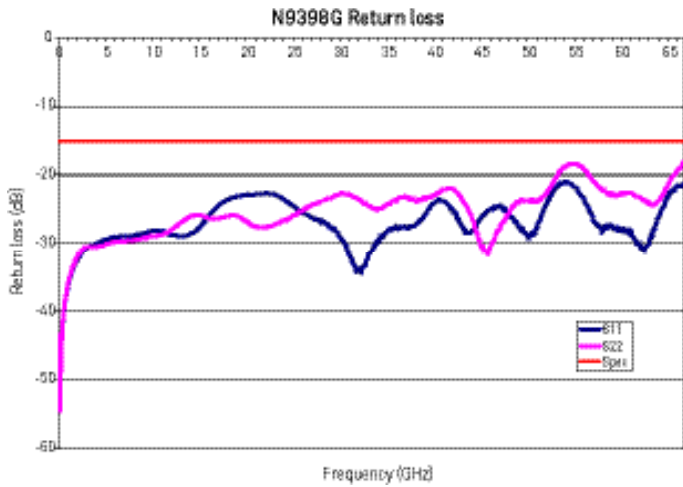
Figure 14. N9398G typical return loss versus frequency
