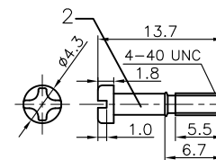
Short BOLT
