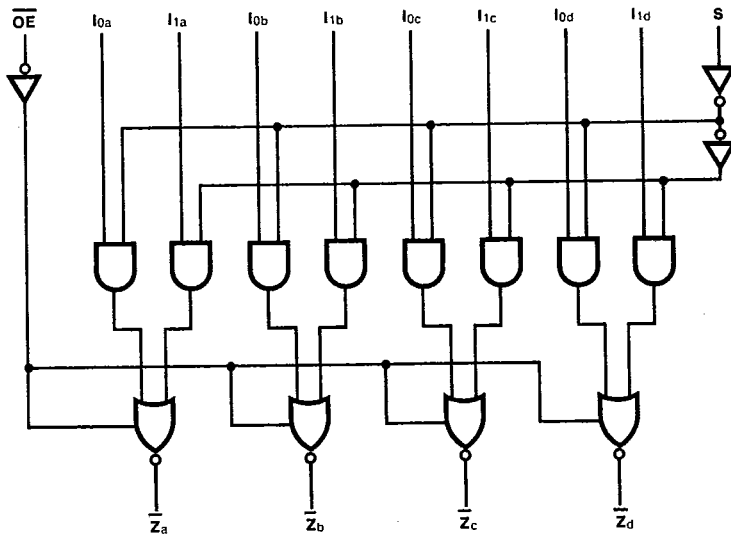
LOGIC DIAGRAM
