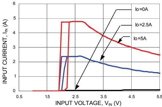
Figure 8. Input voltage vs. Input Current ( V_{out} = 2.5Vdc ).
