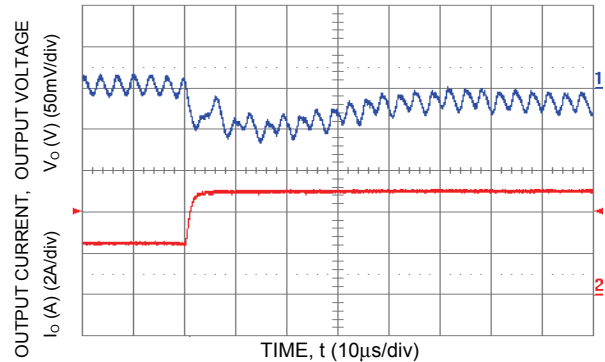
Figure 13. Transient Response to Dynamic Load Change from 50% to 100% of full load ( V_o = 5.0 Vdc , C_{ext} = 2x150 \mu F Polymer Capacitors).
