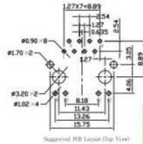
Suggested PCB Layout (Top View)
