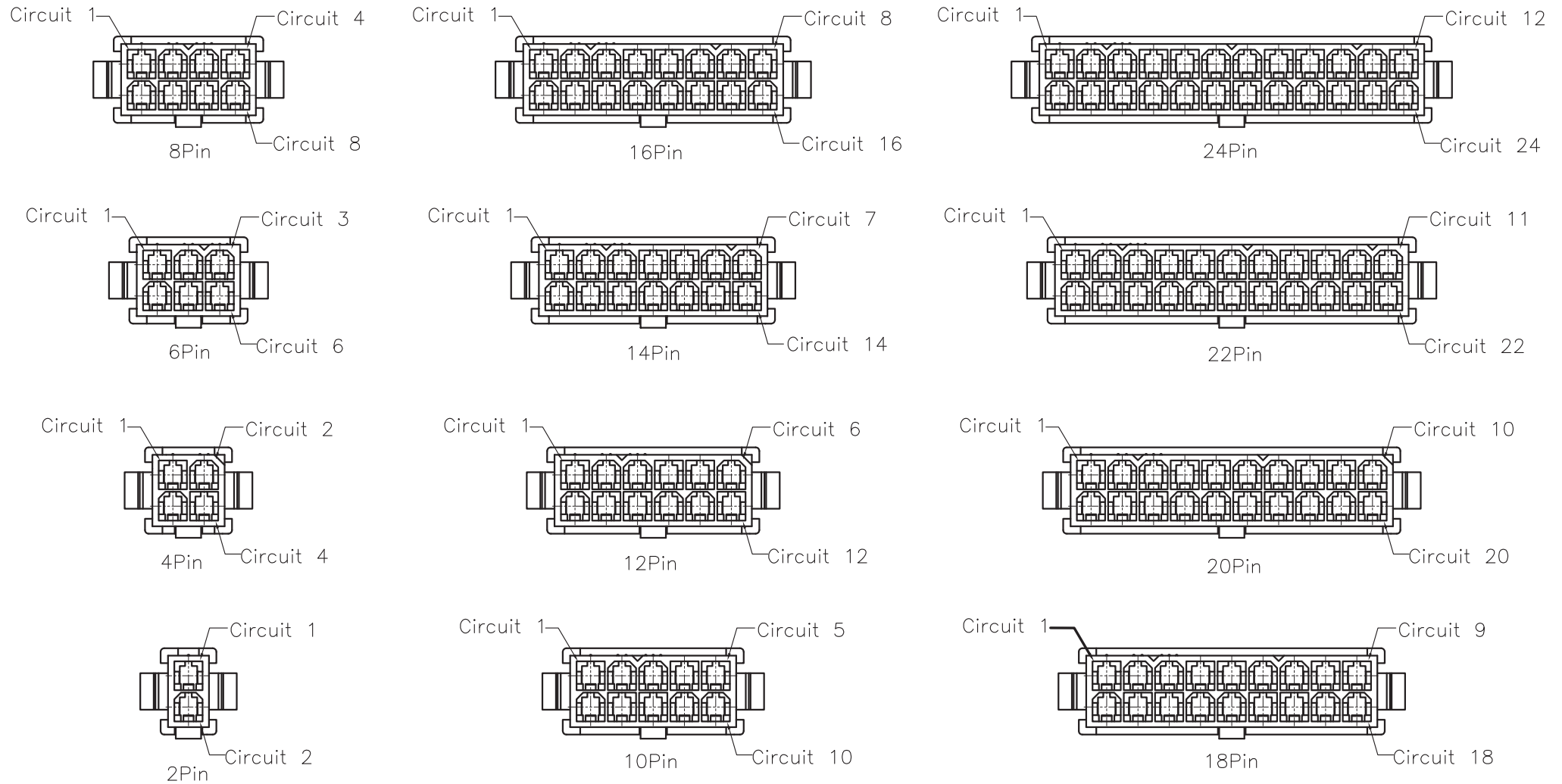
2~24P Protection Key Drawing(Ref.)
