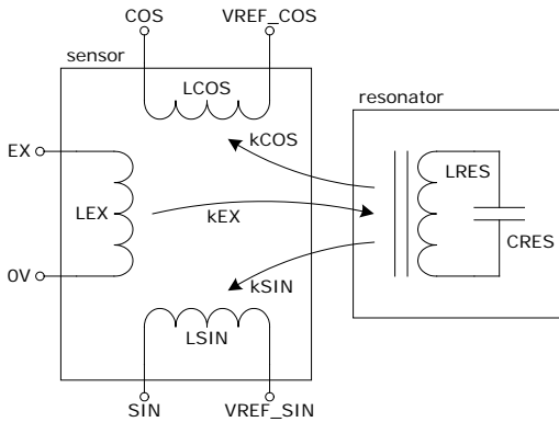
Figure 1 equivalent circuit
