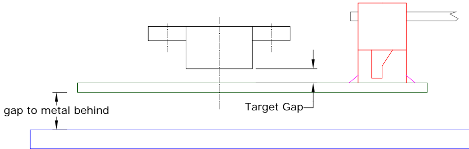
Figure 14 metal behind sensor
