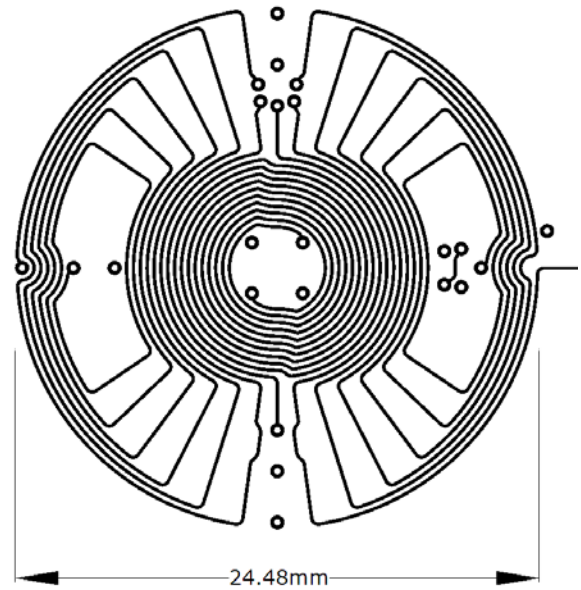
Figure 3: layer 1 sensor pattern
