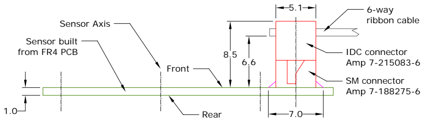
Figure 5 sensor board part number 013-0006 mated with connector 013-6001
