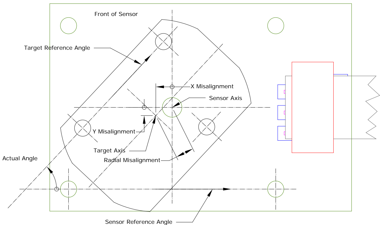
Figure 8 Definition of X, Y and Radial Misalignment, and Actual Angle
