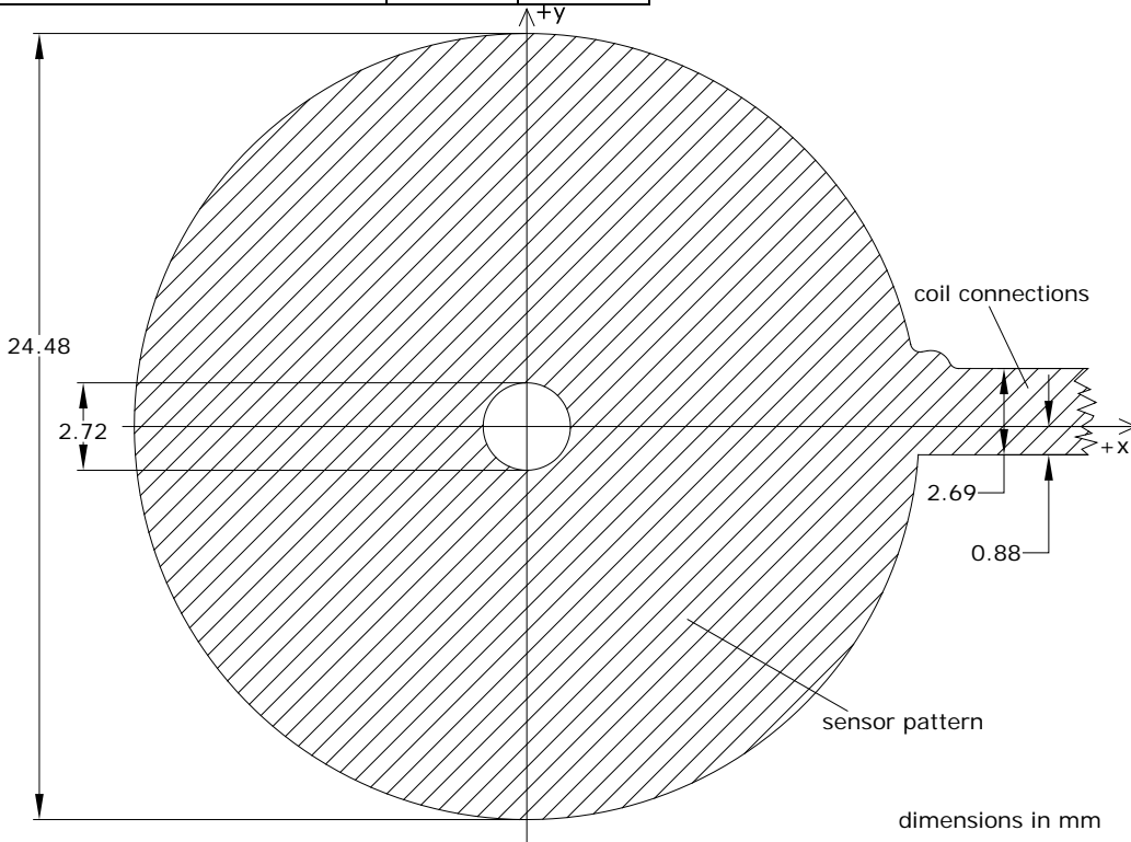
Figure 17 copper extents
