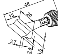
0102WDLF35/SB PowerWell with concave portion, 3.5 mm ø
