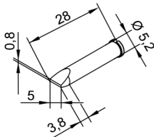
0102CDLF50/SB chisel-shaped, 5.0 mm
