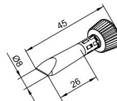
0102CDLF080C/SB chisel-shaped, conical, 8.0 mm
