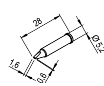
0102CDLF16/SB chisel-shaped, 1.6 mm
