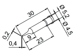
0102CDLF04/SB chisel-shaped, 0.4 mm
