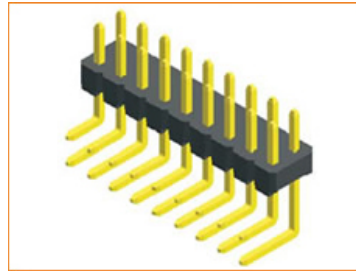
[ 2.54mm Pin Header, Double Row, Right Angle Type , 2*40 Poles ]
