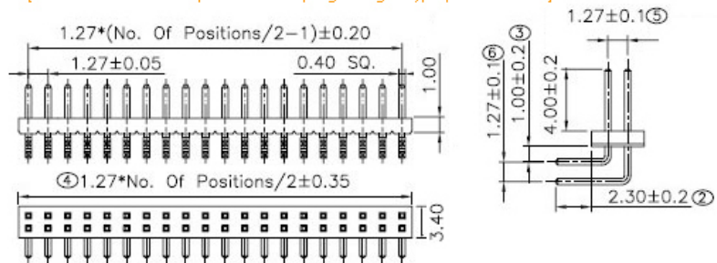
[ 1.27mm Pin Header, Double Row, Right Angle Type , 2*40 Poles ]
