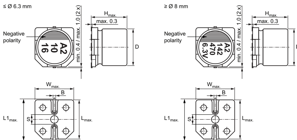
Fig. 2 - Dimensional outline
