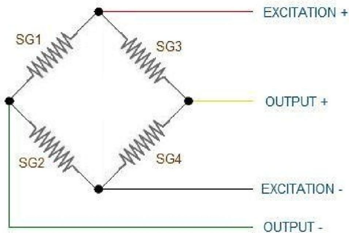
LOAD CELL WIRING
