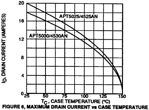
FIGURE 6, MAXIMUM DRAIN CURRENT vs CASE TEMPERATURE
