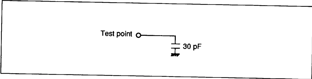
Figure 8 Load Circuit
