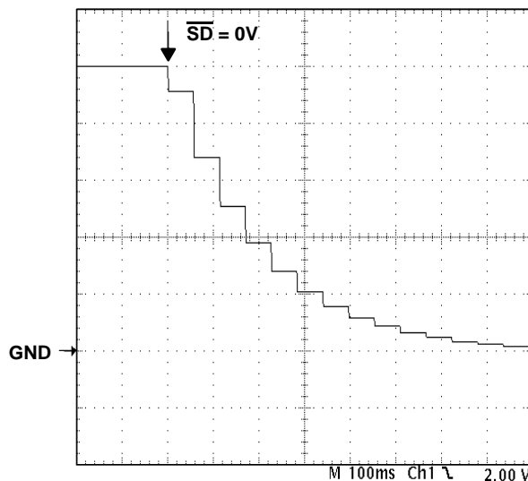
Figure 44. Differential Output With \overline{FADE} (Terminal 30) Held Low
