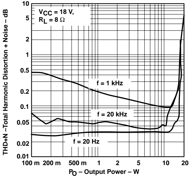
TOTAL HARMONIC DISTORTION + NOISE vs OUTPUT POWER
