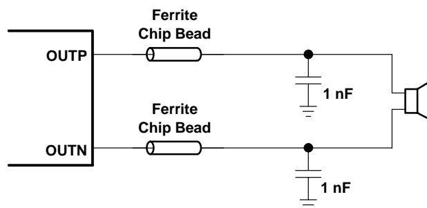
Figure 41. Typical Ferrite Chip Bead Filter (Chip bead example: Fair-Rite 2512067007Y3)
