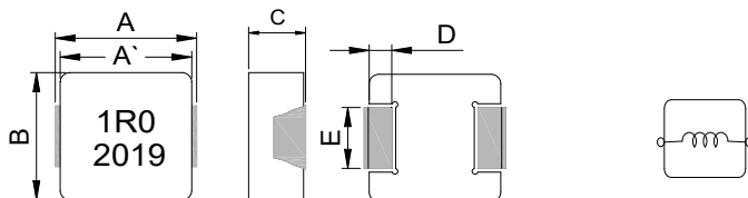
non-leadframe
