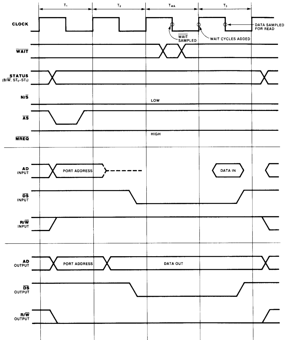
Figure 13. Input/Output Timing
