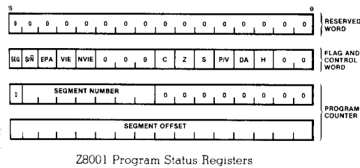
Z8001 Program Status Registers
