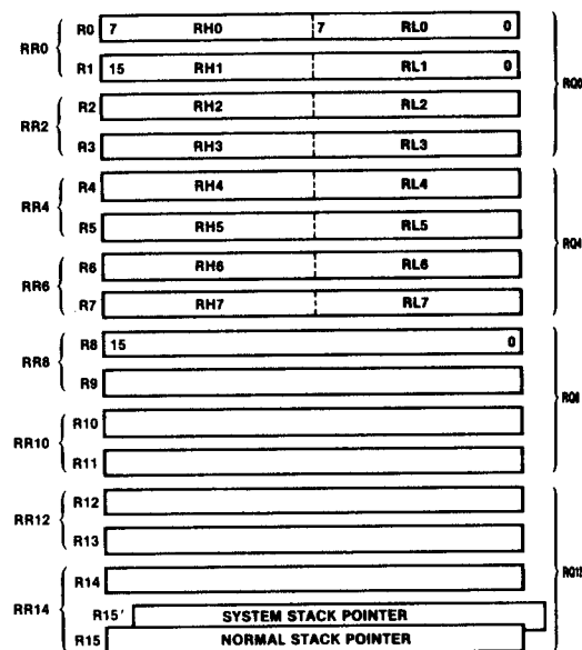
Figure 3. Z8002 General-Purpose Registers
