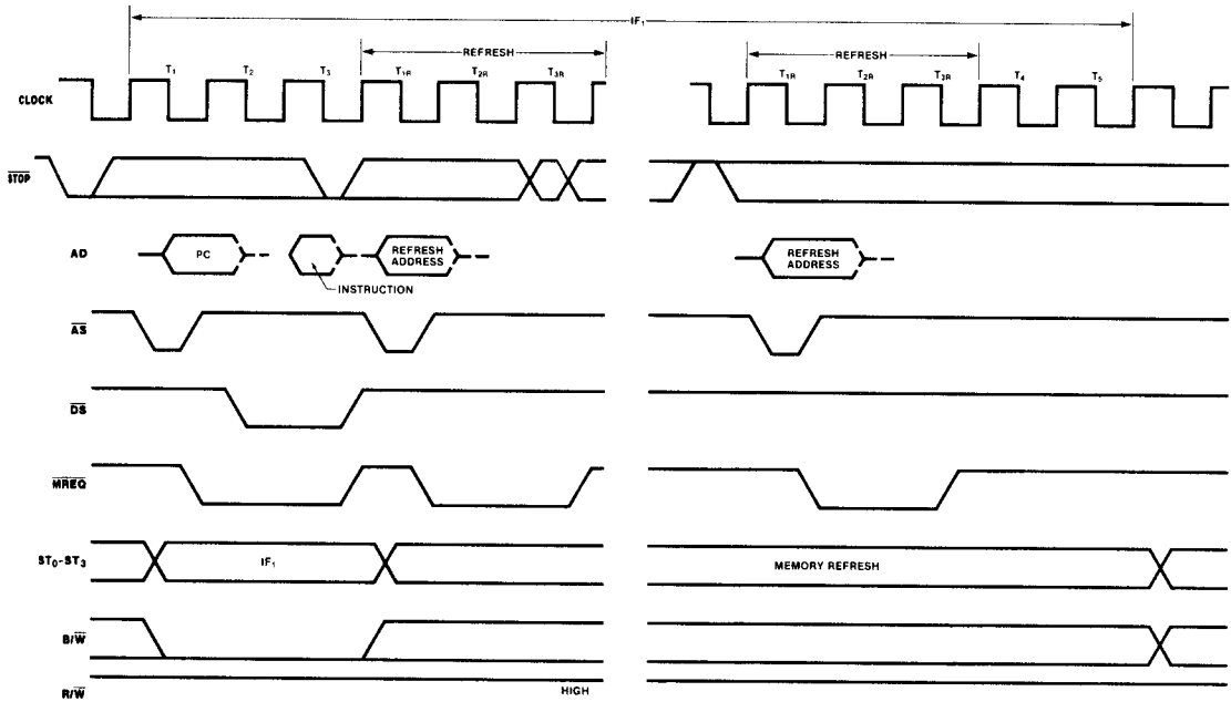
Figure 16. Stop Timing
