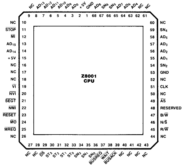
Figure 10b. 68-pin Chip Carrier, Pin Assignments
