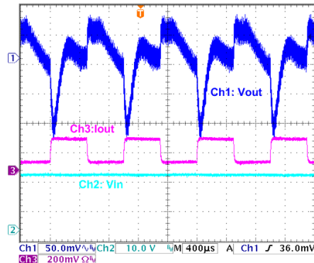
Load Transient (HT7463B, I_{OUT}=50mA to 200mA )
