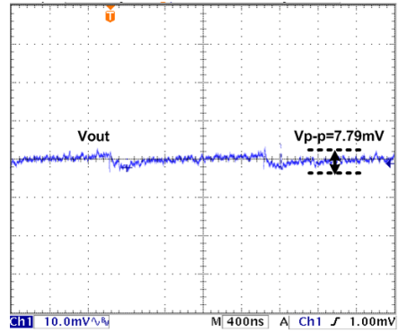
Output Ripple (HT7463B, I_{OUT}=400mA )
