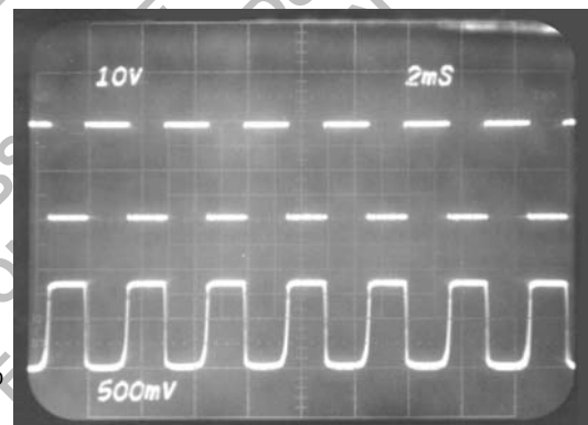
Figure 7. Output Pulse for an 8 Tooth Gear
