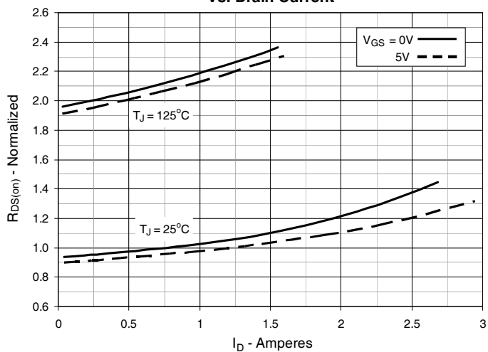
Fig. 8. R_{DS(on)} Normalized to I_D = 0.8A Value vs. Drain Current
