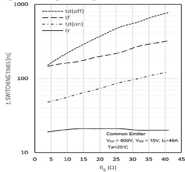
Fig. 3 Switching times vs. gate resistor
