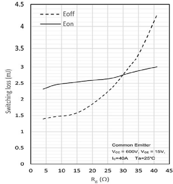
Fig. 5 Switching loss vs. gate resistor
