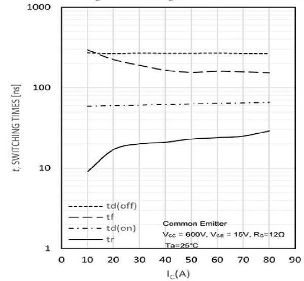
Fig. 4 Switching times vs. collector current
