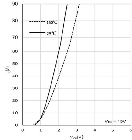
Fig. 2 Saturation voltage characteristics
