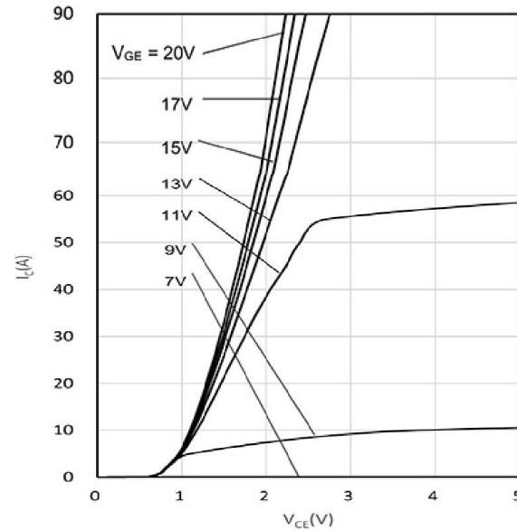
Fig. 1 Output characteristics
