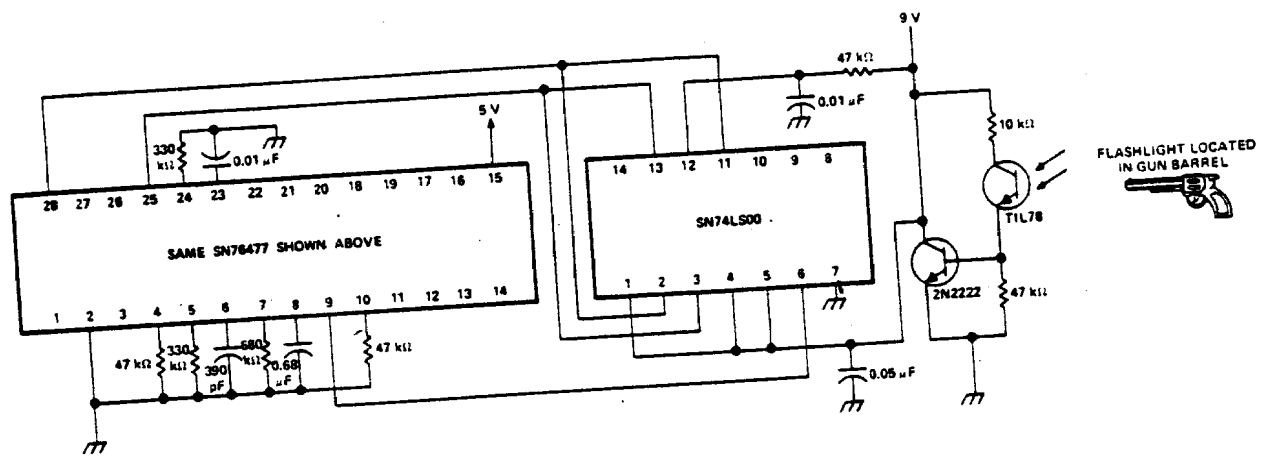
ADDITIONAL CIRCUITRY FOR SILENCER AND GUN SHOT (FOR USE WITH BIRD SOUNDS ABOVE)
