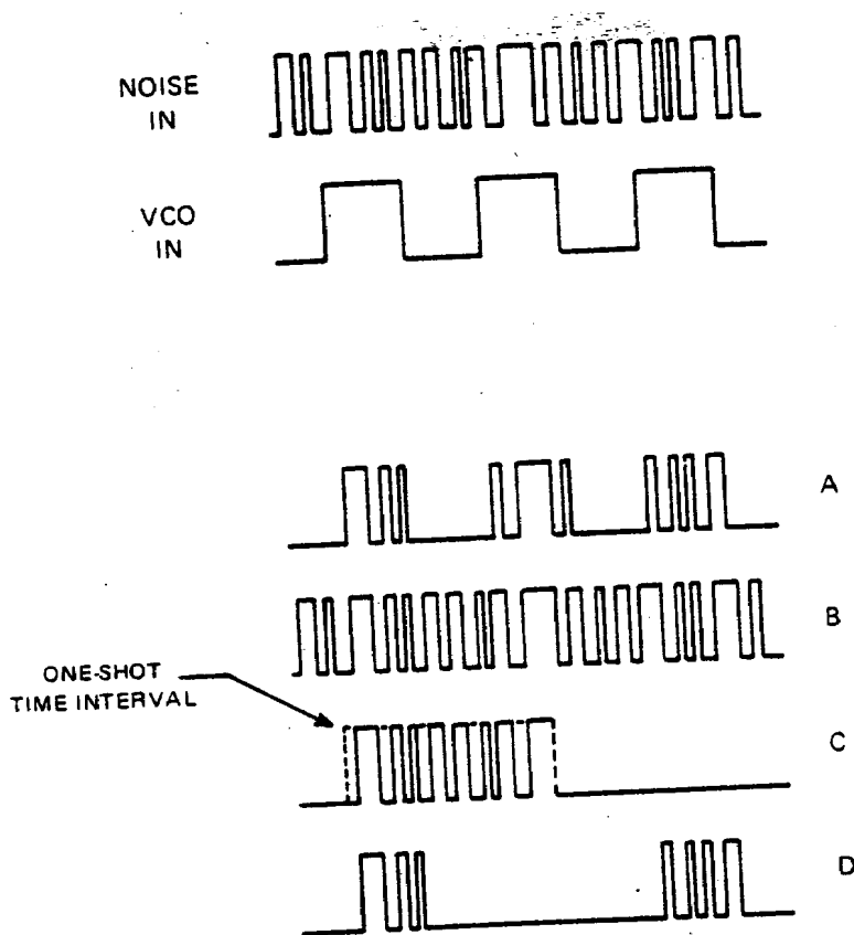
FIGURE 4: EXAMPLES OF THE FOUR SELECTABLE ENVELOPES USING NOISE AS MIXER OUTPUT: (A) VCO, (B) MIXER ONLY, (C) ONE-SHOT, (D) VCO WITH ALTERNATING CYCLES.
