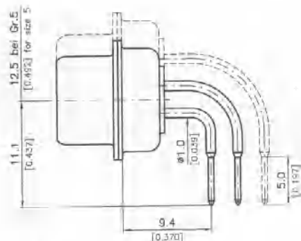
Contact design Kontaktvariante
