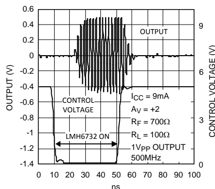
Figure 2. Turn-On/Off Characteristics
