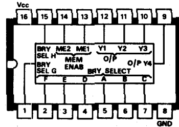
C36 DM8574N 1024-bit programmable ROM (pROM) (Tri-state)
