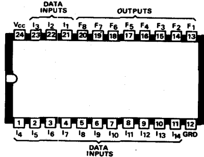
C37 DM8575N Programmable logic array (Active)
