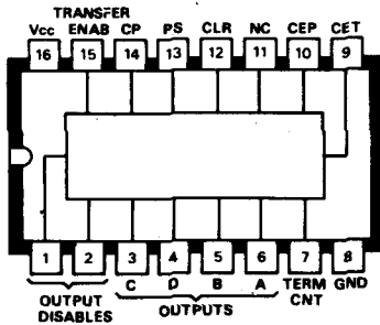
C32 DM8554N Binary counter/latch (Tri-state)
