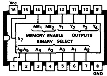
C35 DM8573N 1024-bit programmable ROM (pROM)
