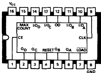
C34 DM8556N Tri-State Programmable Binary Counter
