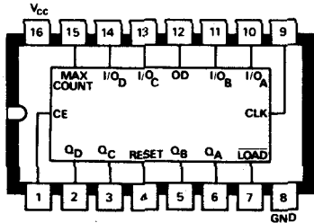
C33 DM8555N Tri-State Programmable Decade Counter
