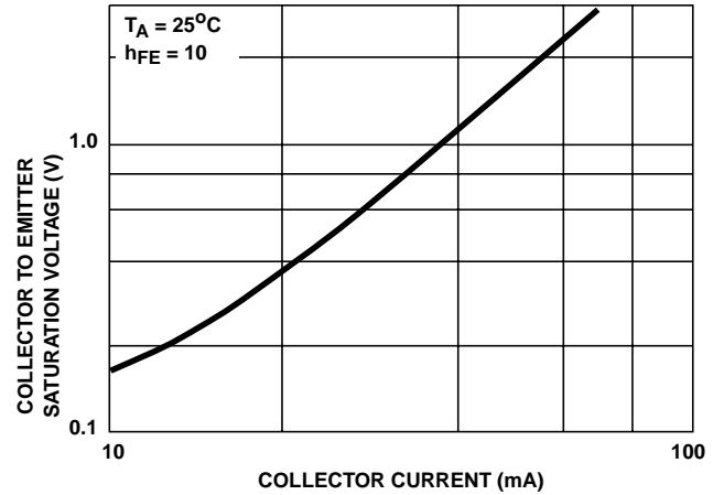
FIGURE 24. V_{CE SAT} vs I_C FOR ANY TRANSISTOR
