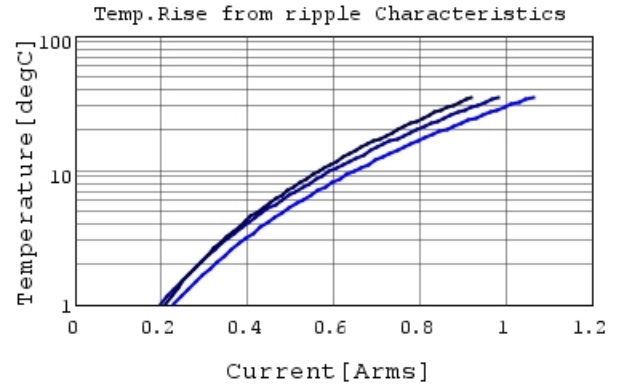
GRM1552C1H120GA01 Temp.rise — 500MHz
