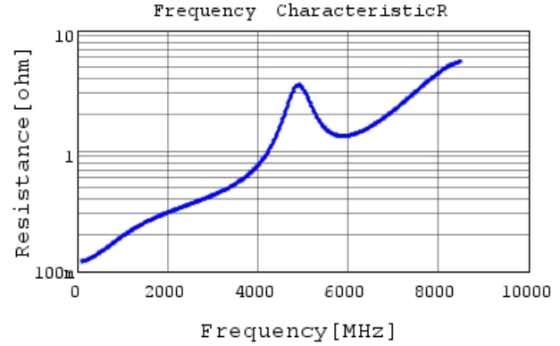
GRM1552C1H120GA01 R DCOV, 20degC
