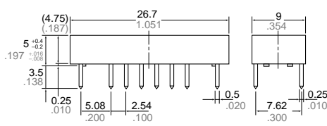
External dimensions Standard PC board terminal
