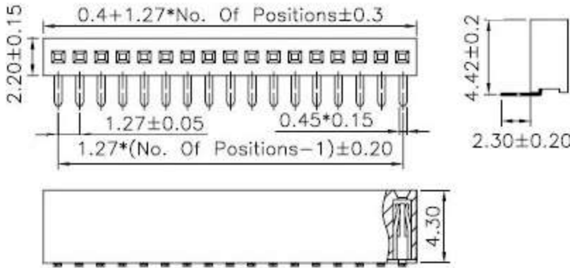
[ 1.27 Female Header, 1 Rows, Right Angle Type , 1*40 Poles ]
