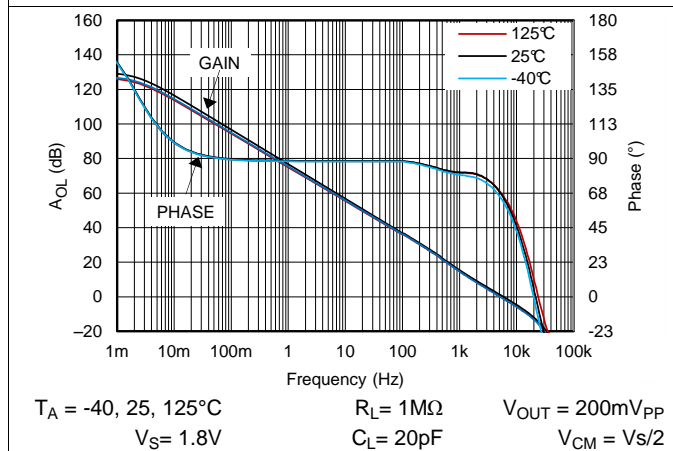
Figure 33. Open Loop Gain and Phase, 1.8V, 1 MΩ Load
