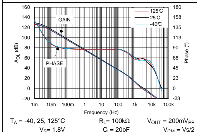
Figure 35. Open Loop Gain and Phase, 1.8V, 100kΩ Load
