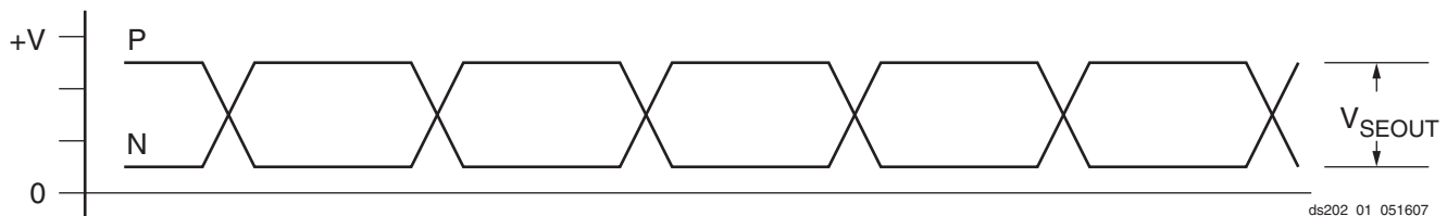
Figure 6: Single-Ended Output Voltage Swing
