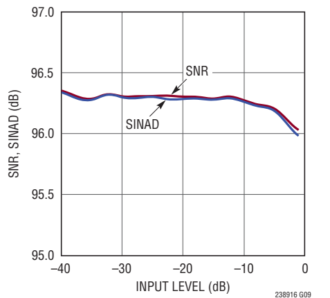
SNR, SINAD vs Input Level, f_{IN} = 2\text{kHz}
