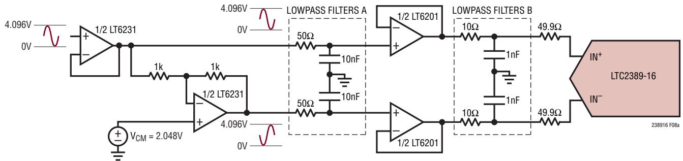
Figure 8a. LT6231 Converting a 0V to 4.096V Single-Ended Signal to a ±4.096V Fully-Differential Signal Followed by LT6201 Buffering Fully-Differential Signal
