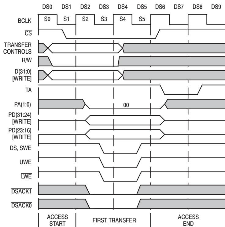
Figure 30. 16-Bit '040 WRITE to 32-Bit Peripheral Example (PA1=0)
