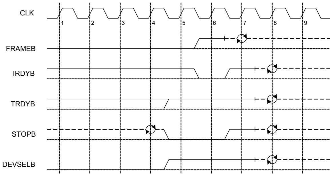
Figure 25. Target Initiated Termination - Abort
