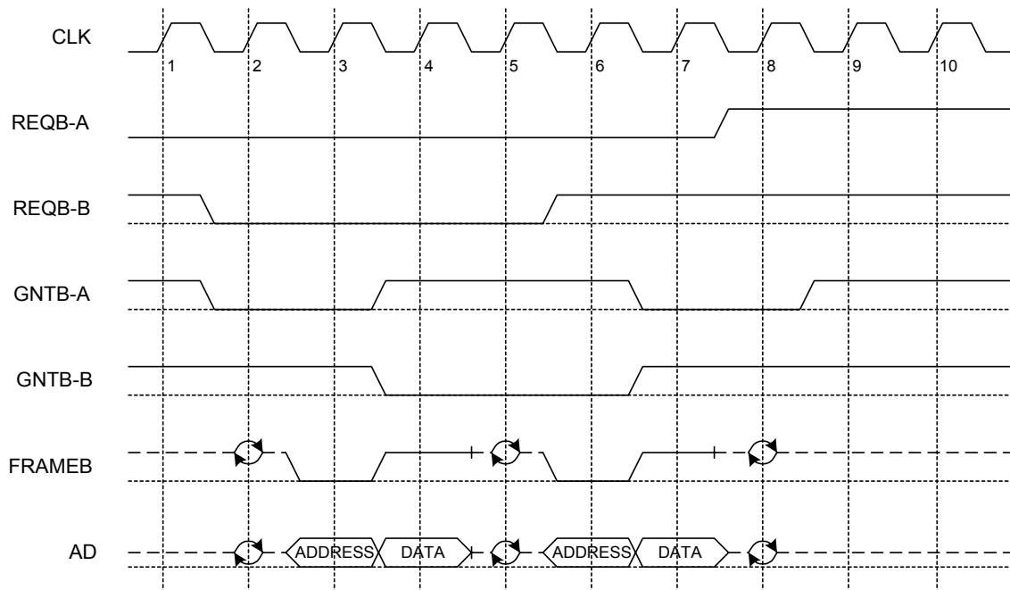
Figure 21. Bus Arbitration
