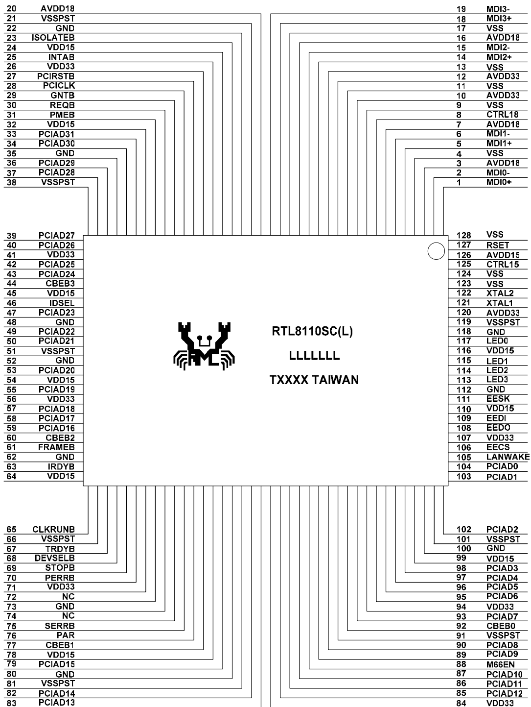
Figure 1. 128-Pin (L)QFP Pin Assignments
