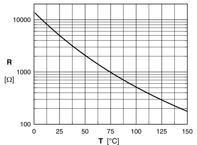
Fig. 13 Typ. thermistor resistance vs. temperature
